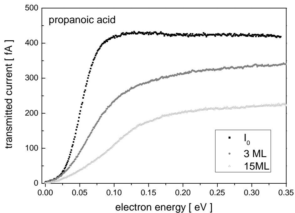
Figure 6: Transmitted current vs. electron energy for propanoic acid at 130K. The top curve is for bare tantalum, and the curves refer successively to 3 and 15 monolayers.
