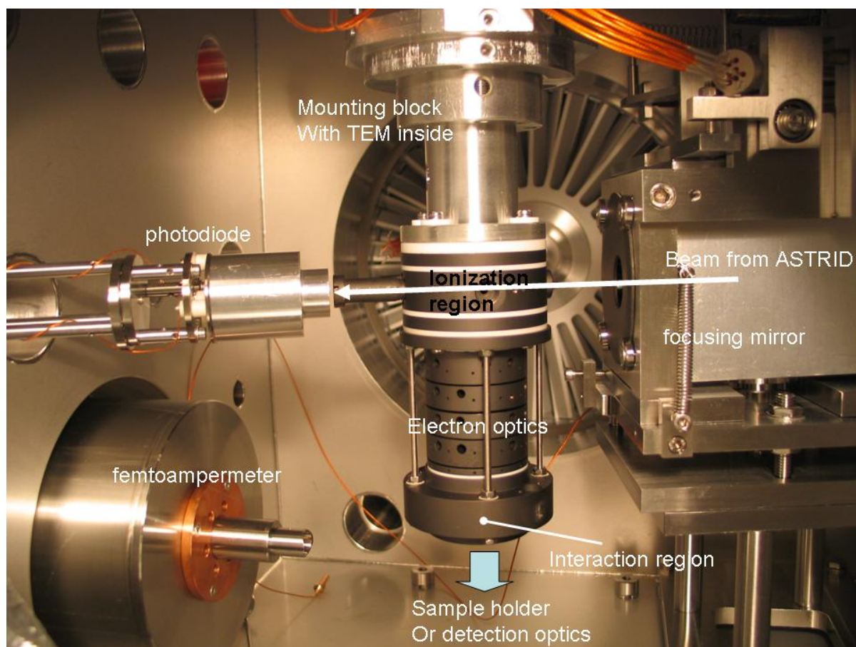
Figure 1: The experimental system.
