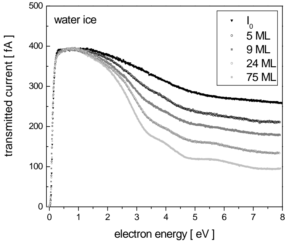
Figure 3: Transmitted current vs. electron energy for polycrystalline water ice at 130K. The top curve is for bare tantalum, and the curves refer successively to 5, 9, 24 and 75 monolayers.
