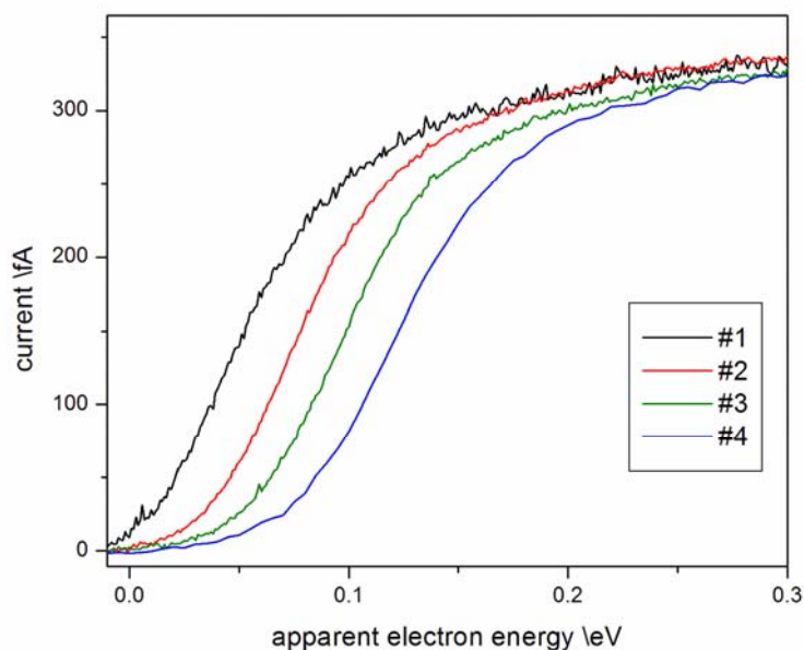
Figure 5: Successive scans through a 3ML sample of propanoic acid at 130.
