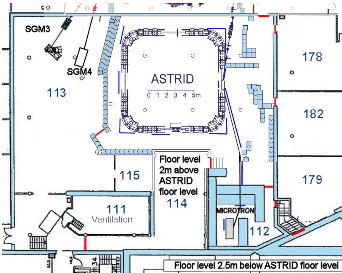
Fig. 3.1: The ASTRID ring hall with the existing (February 2020) concrete walls shown in light blue. Lead shielding is shown in dark blue. North is upwards in the figure.
